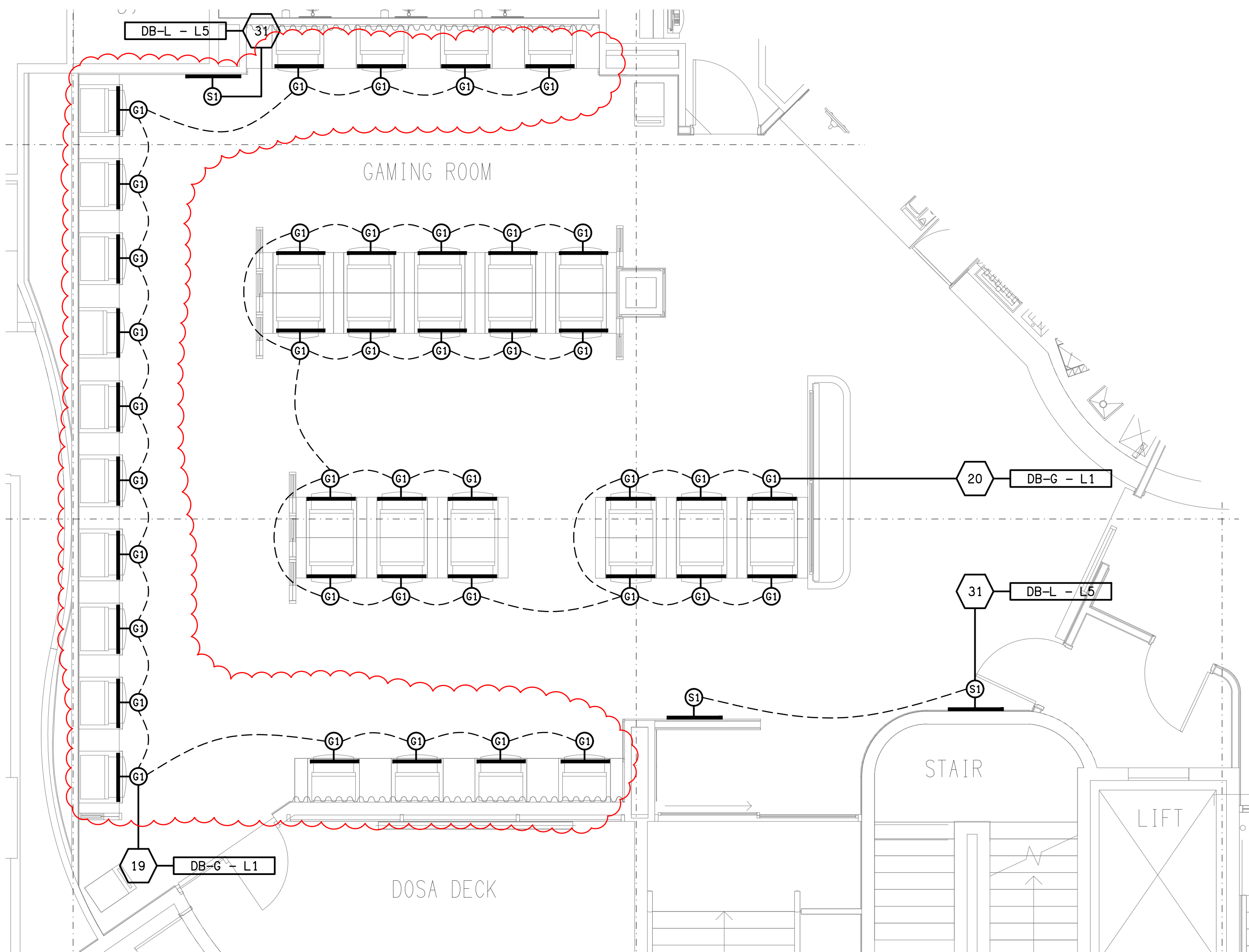
GAMING ROOM LIGHTING PLAN SCALE 1:50
